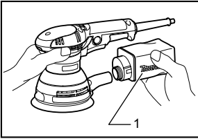
1. Dust bag
