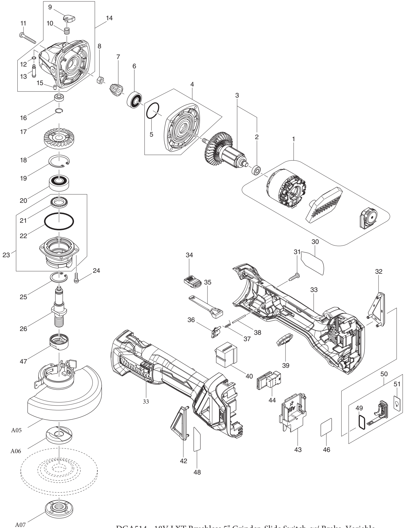
DGA514 - 18V LXT Brushless 5" Grinder, Slide Switch, w/ Brake, Variable Speed, Bluetooth
